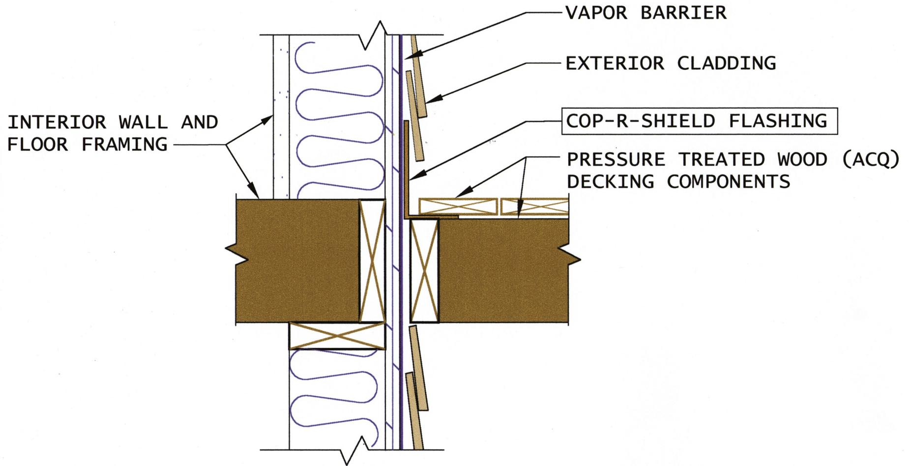
DECK FLASHING DETAIL
