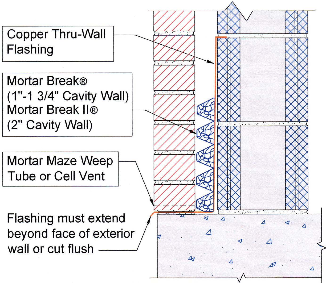
Mortar Break® Detail
