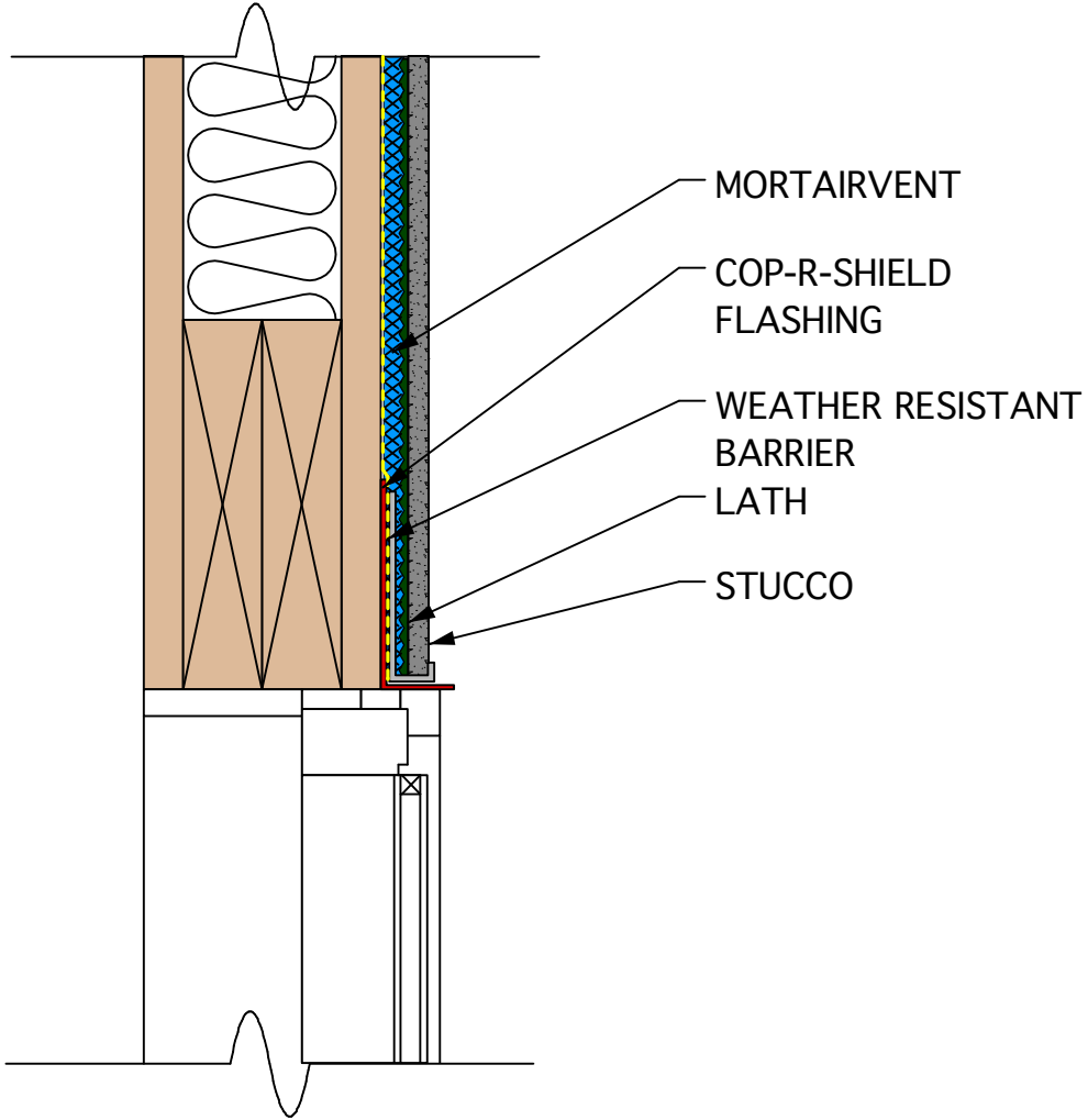
WINDOW HEAD
