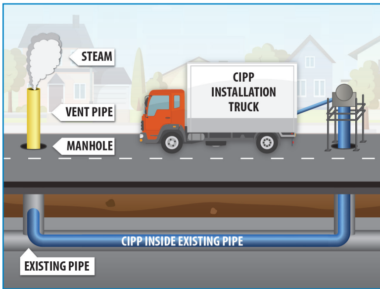
Example of the CIPP installation process.
