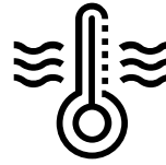
Rising Temperatures
