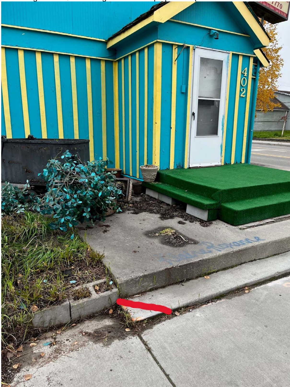
Figure 8: Sawcut Existing Step at Aloha Grill (5 th /Noble)
