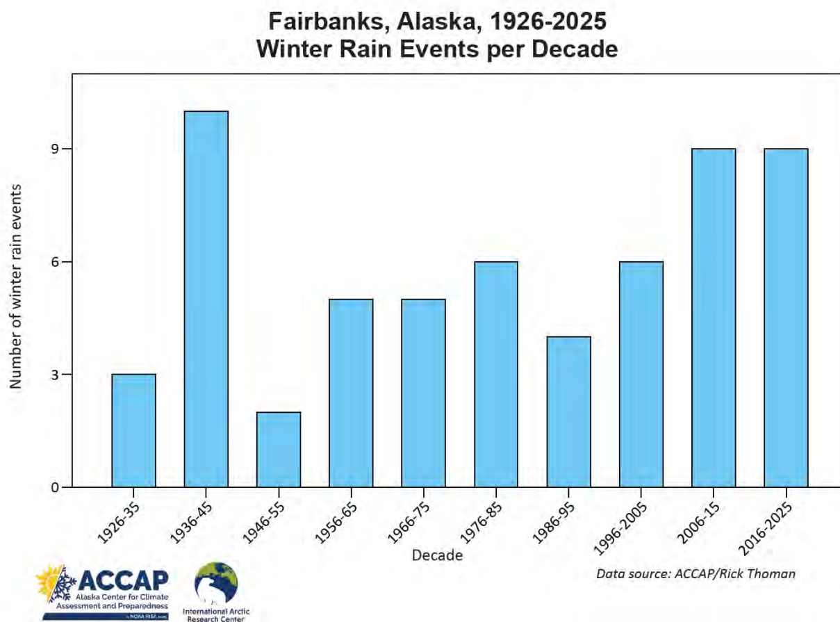
Figure 6-5: Freezing Rain and Ice Accretion in Interior Alaska
