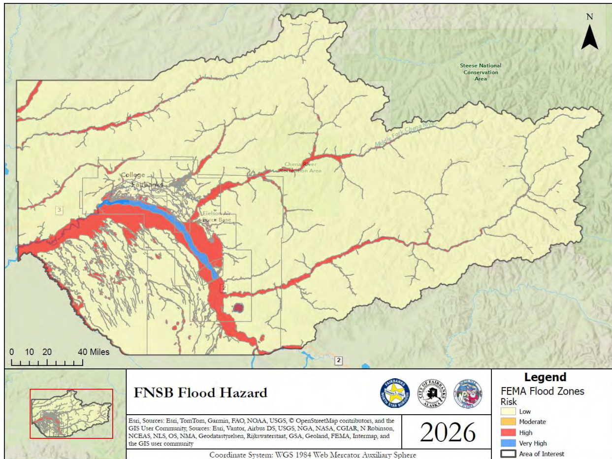
Figure 7-1: Map of Flood Hazard Extent - Borough
