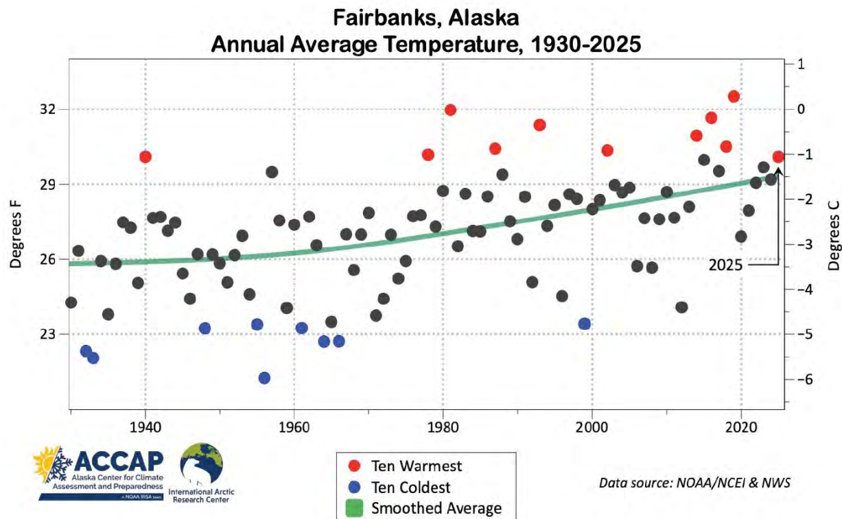
Figure 6-6: Annual Average Temperature – Fairbanks Area
