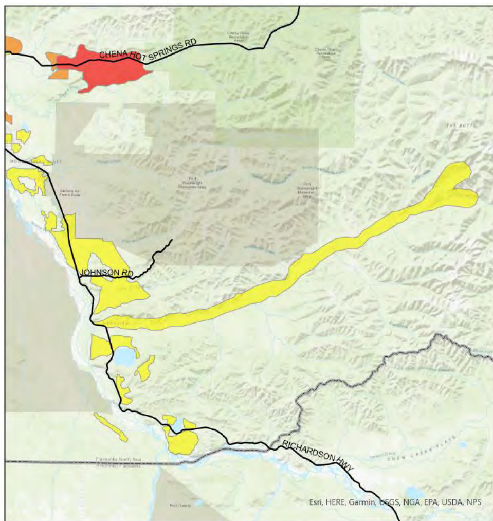
Figure 5-9: Map of FNSB Wildland Fire Zones of Concern – Eastern Population
