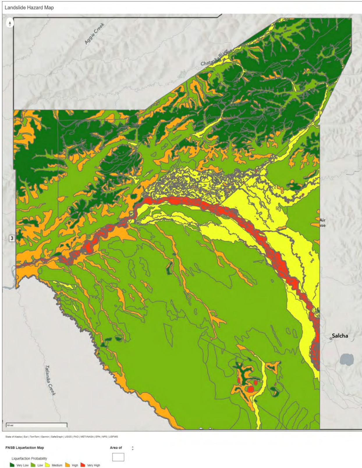
Figure 9-3: Map of Liquefaction Susceptibility
