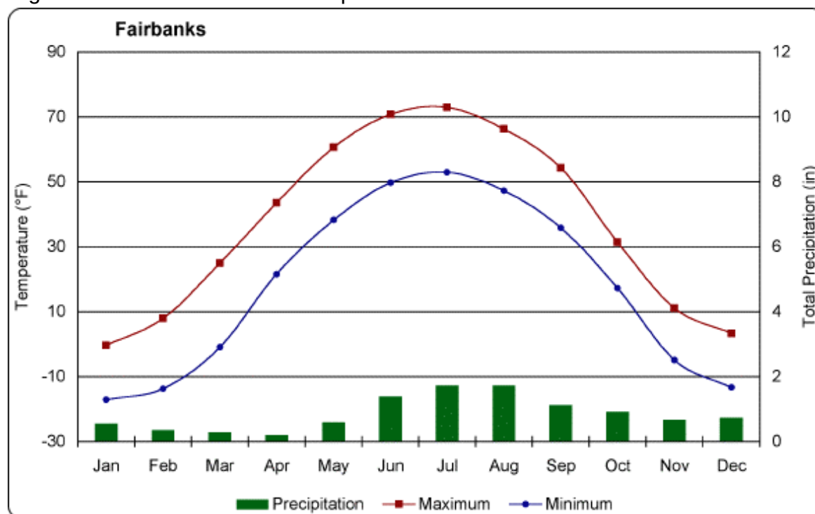
Figure 6-3: Mean Annual Temperature Trends – FNSB
