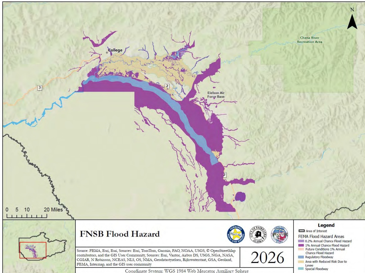
Figure 7-2: Map of Flood Hazard Extent - Urban Core
