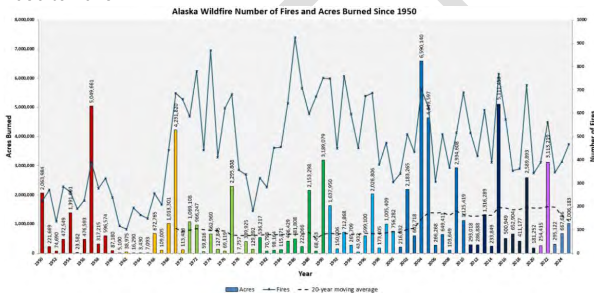
Figure 5-7: Alaska Wildfire Number of Fires and Acres Burned from 1950 to 2025.
