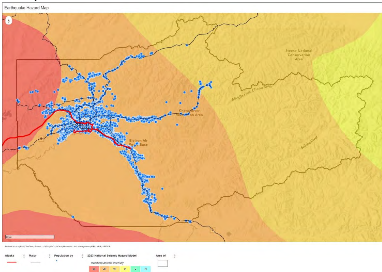
Figure 8-2: Map of Seismic Hazard Intensity with Population and Structure Overlay - FNSB
