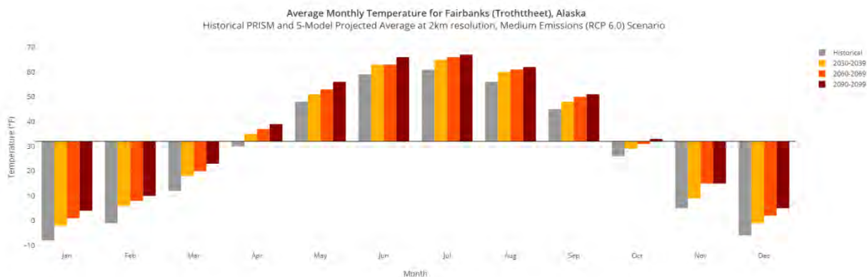
Figure 6-7: Average Monthly Temperature – Fairbanks
