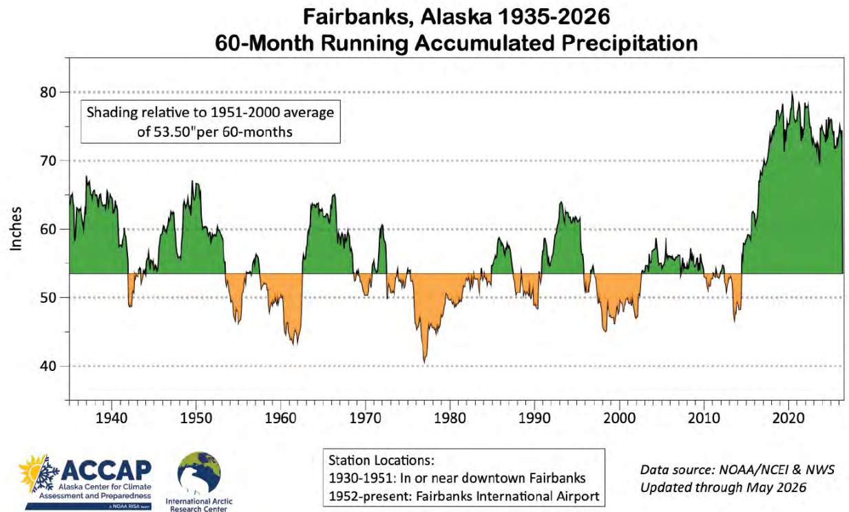
Figure 6-8: Five-Year Running Precipitation Departure – FNSB
