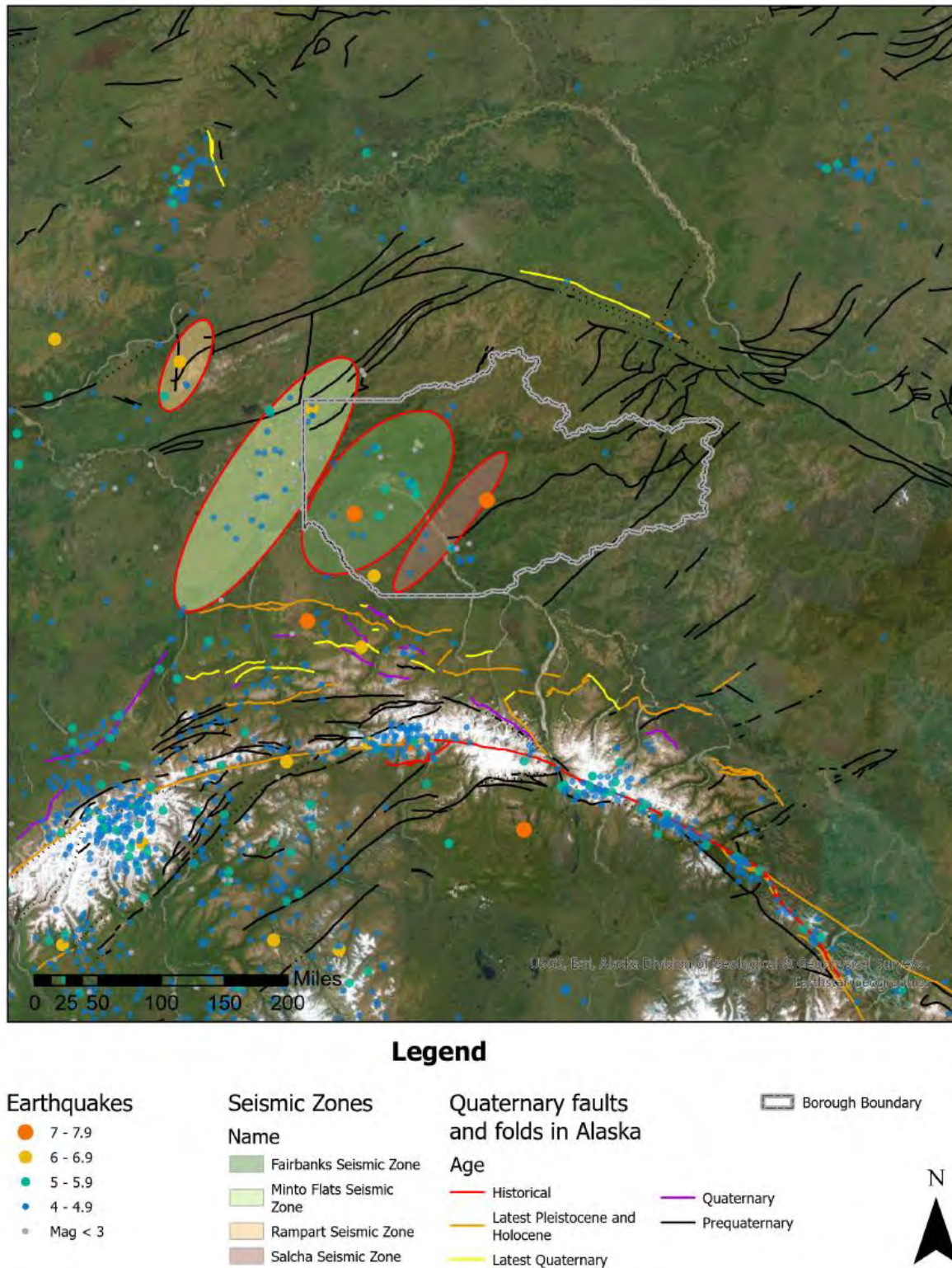
Figure 8-3: Map of Historical Regional Seismicity
