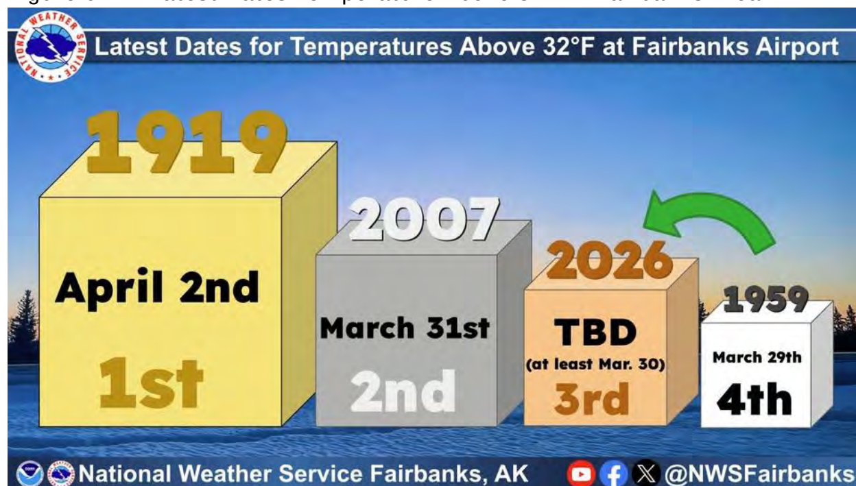
Figure 6-11: Latest Dates Temperature Above 32°F – Fairbanks Area
