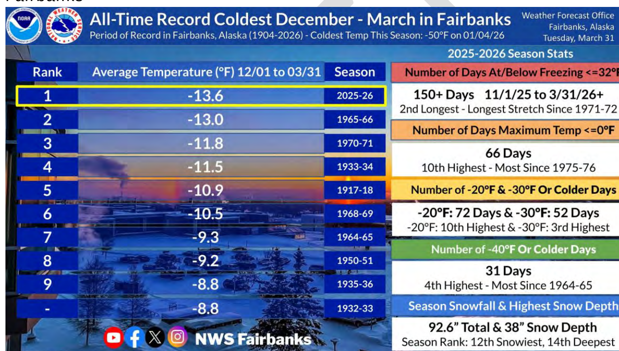
Figure 6-4: 2025-2026 All-Time Record Coldest December-March in Fairbanks
