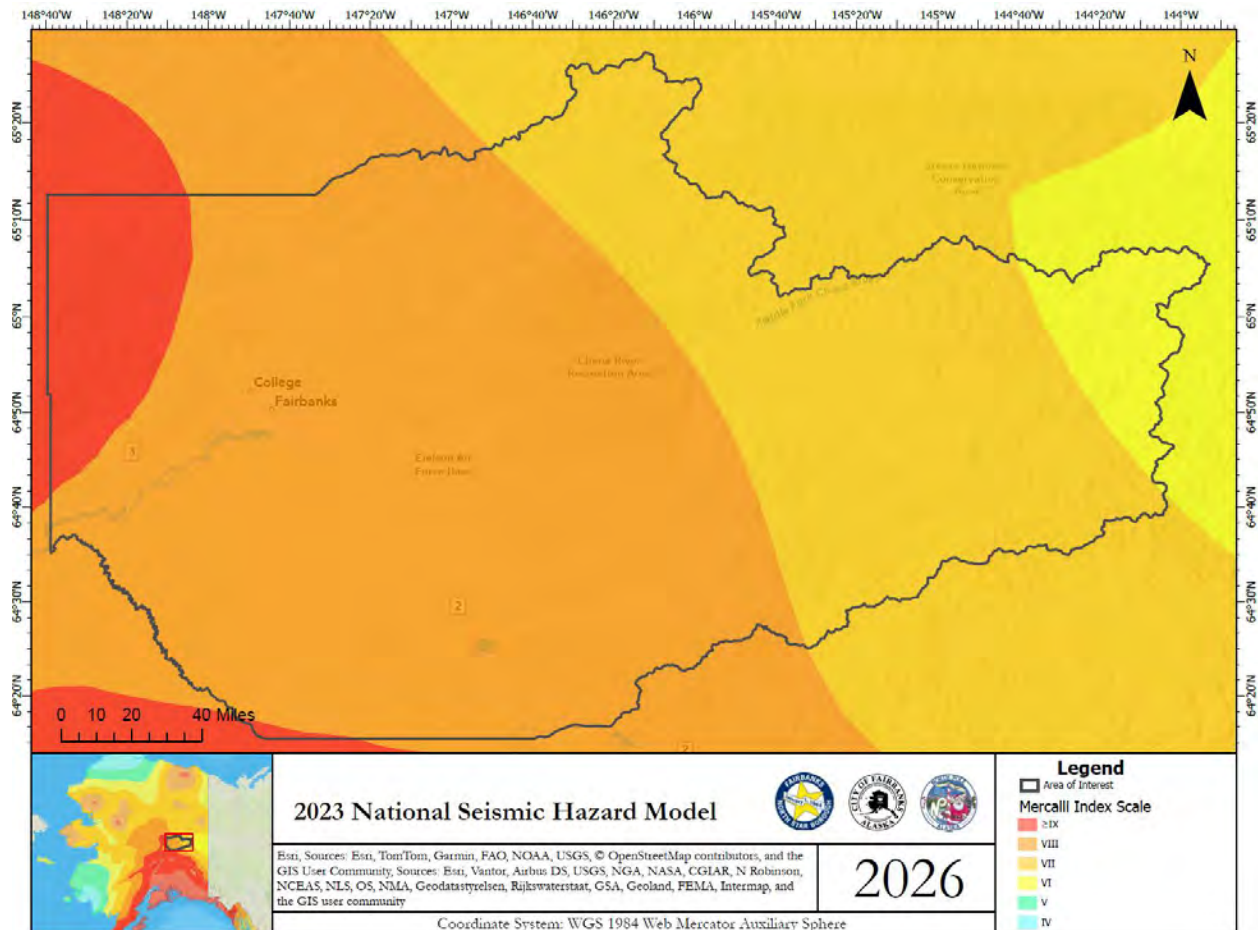
Figure 8-1: Map of Seismic Hazard Intensity – FNSB (Modified Mercalli Intensity)
