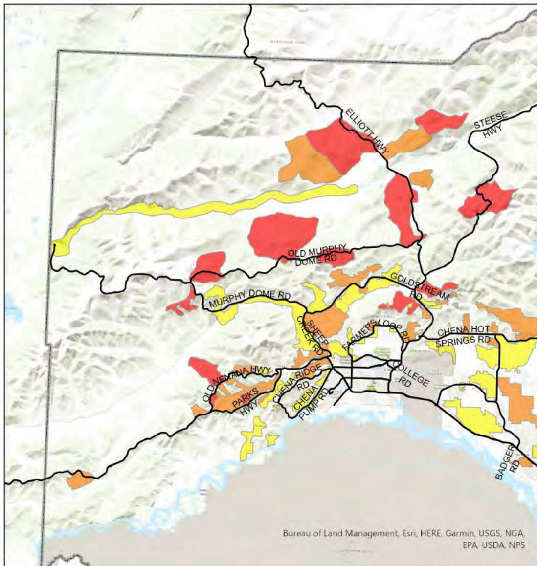
Figure 5-8: Map of FNSB Wildland Fire Zones of Concern – Western Population
