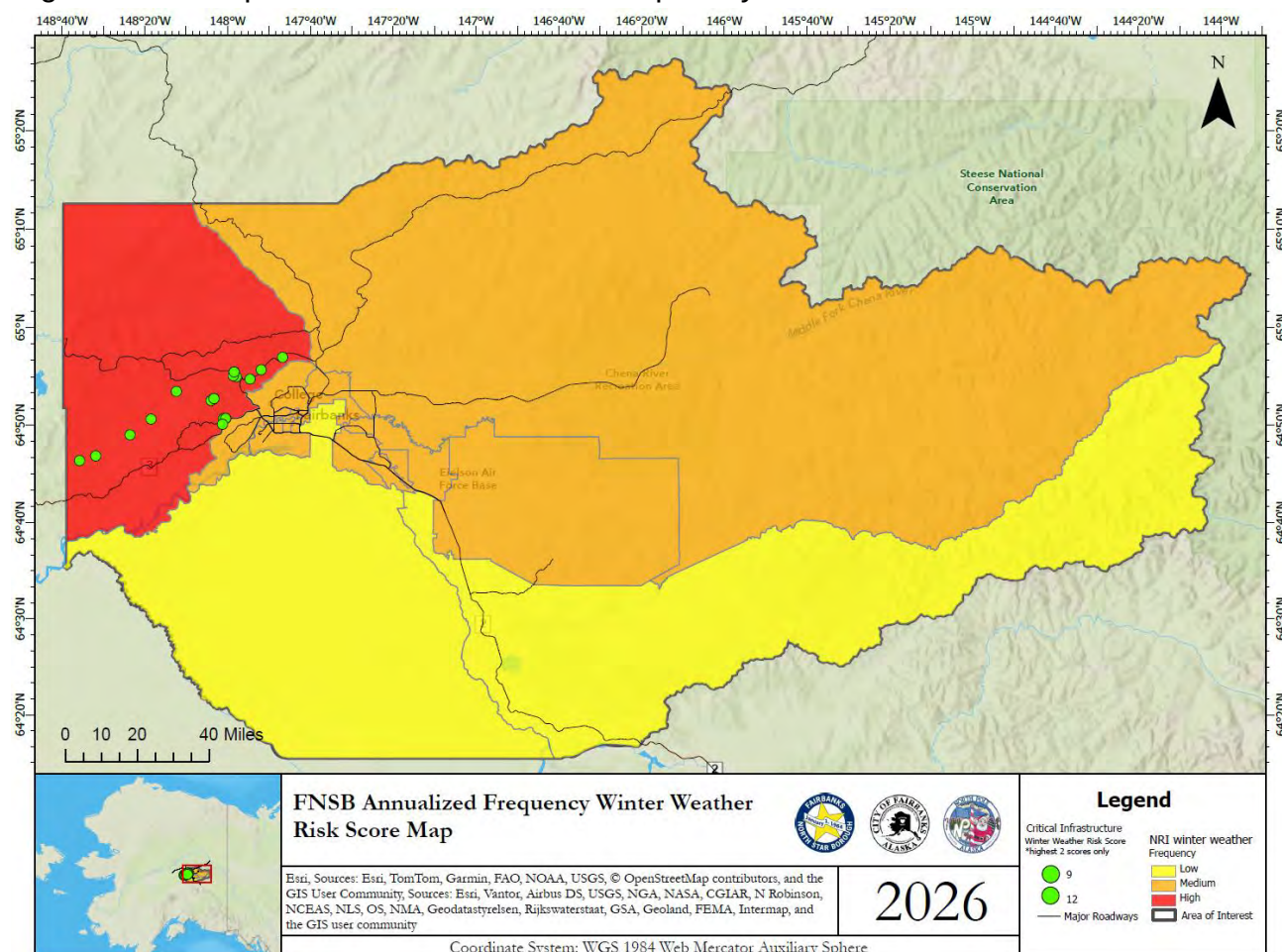
Figure 4-7: Map of FNSB Annualized Frequency Winter Weather Risk Score
