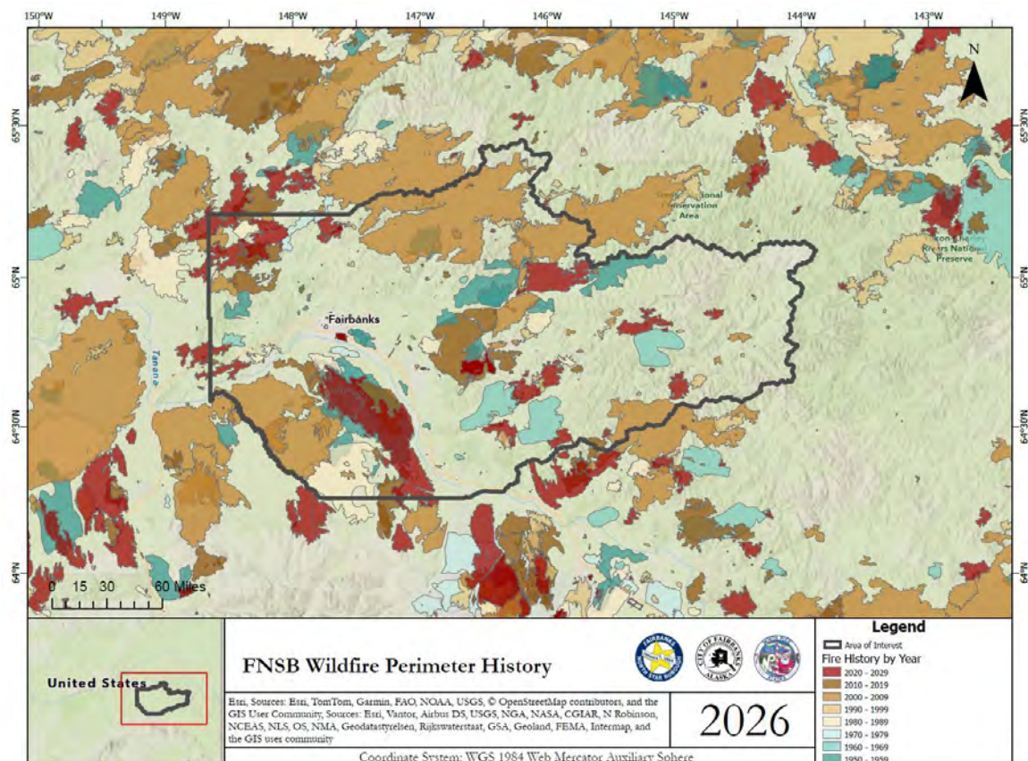
Figure 5-2: Map of FNSB Fire History
