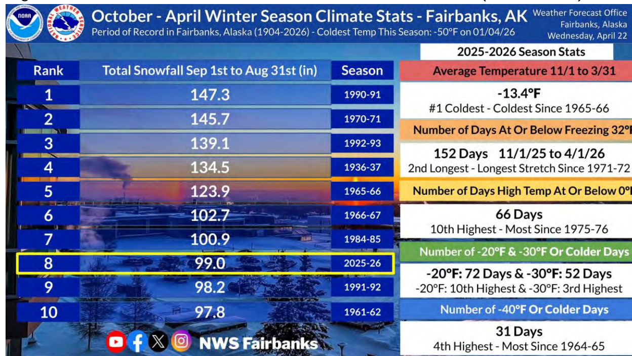
Figure 6-10: Winter Season Climate Statistics – Fairbanks (2025-2026)
