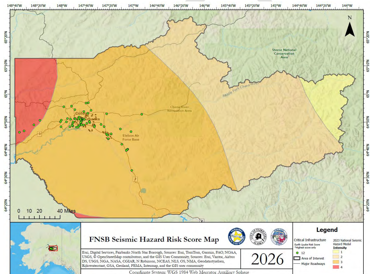
Figure 4-9: Map of FNSB Seismic Hazard Risk Score
