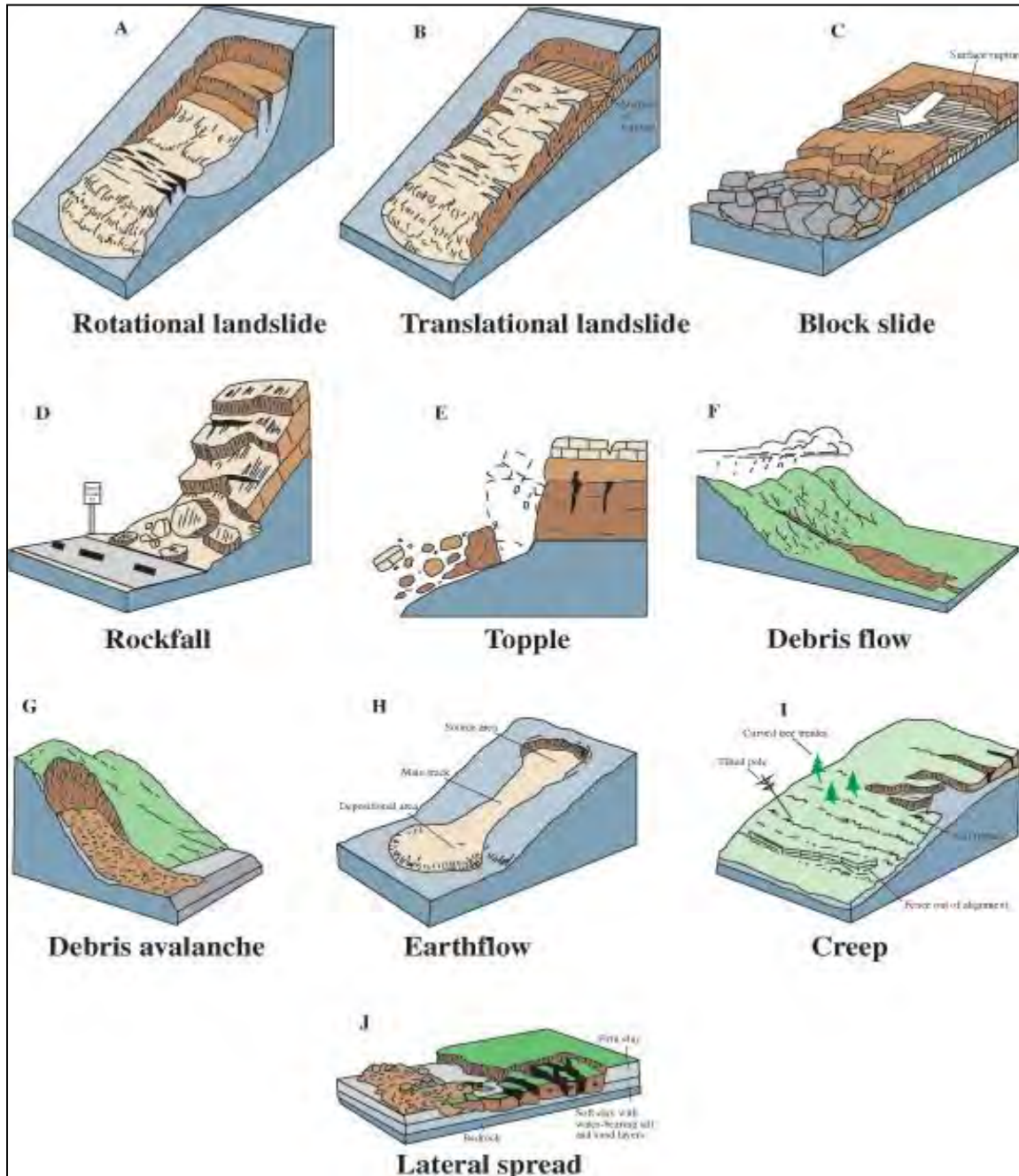
Figure 9-1: Landslide Classifications
