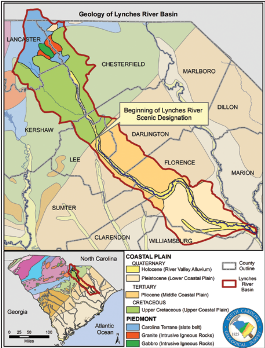
Generalized geology of the Lynchses River Basin. For more information, visit the South Carolina Geological Survey of the SCDNR at www.dnr.sc.gov/geology .
