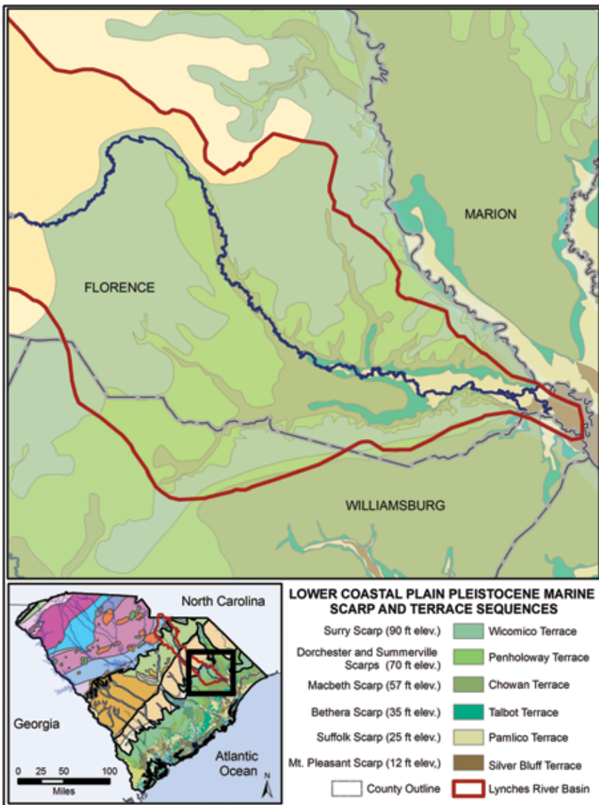
Projected boundaries for Pleistocene marine terrace and scarp sequences in the Lower Coastal Plain area of the Lynchies River Basin.
