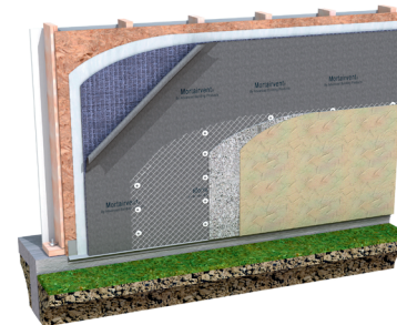
Stucco Cladding
